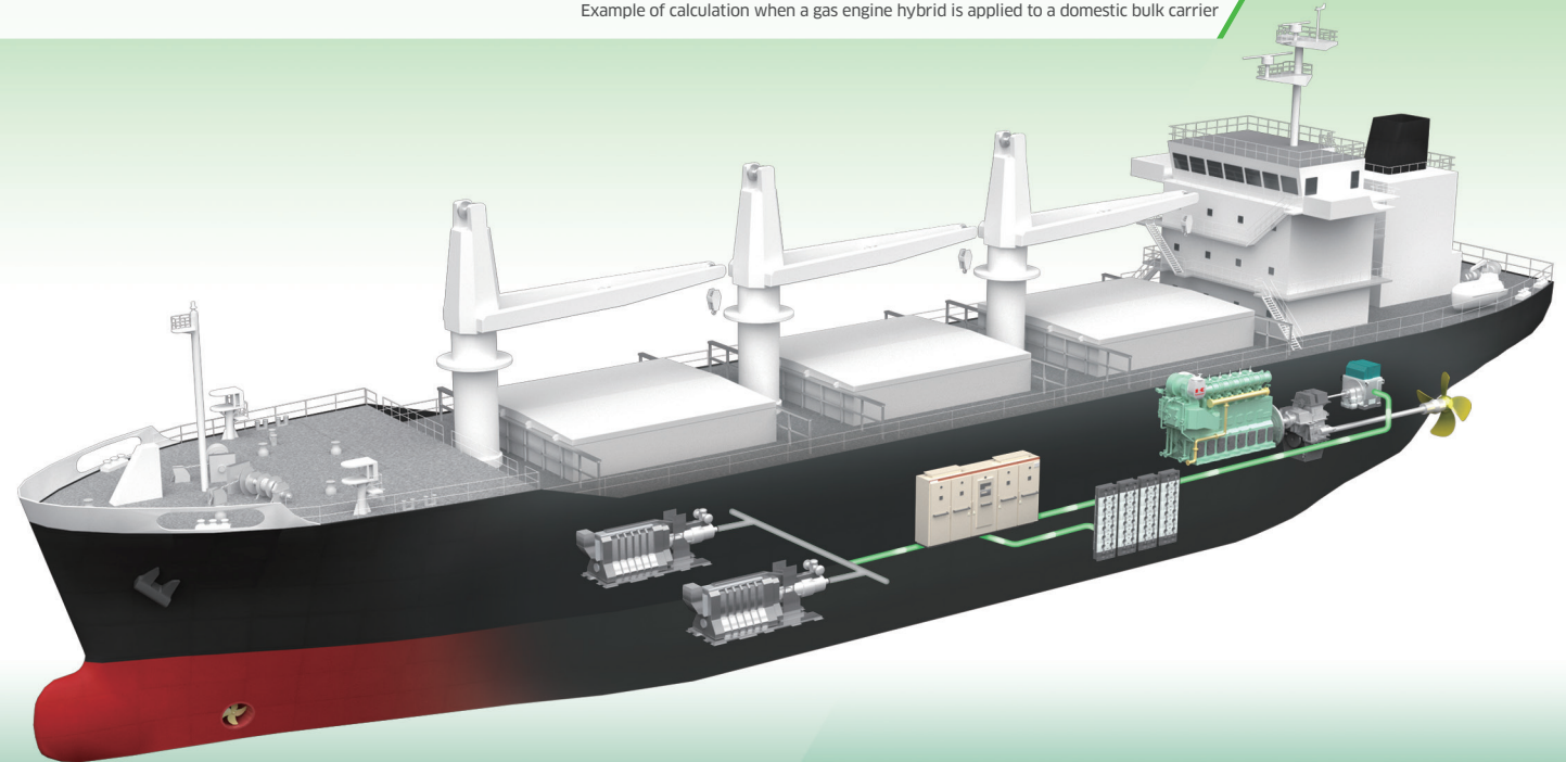
Example of calculation when a gas engine hybrid is applied to a domestic bulk carrier
