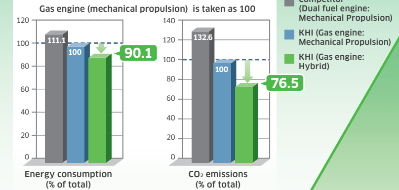
Example of calculation when a gas engine hybrid is applied to a domestic bulk carrier
